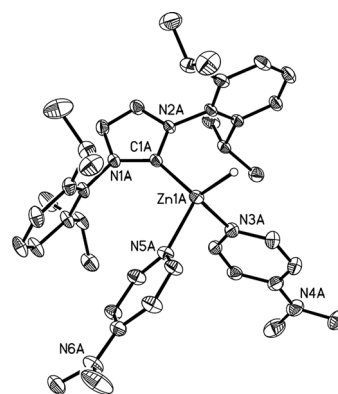
Figure 4. Molecular structure of [\text{IPr-ZnH}(\text{DMAP})_2]\text{OTf} ( 5 ) with thermal ellipsoids at the 30% probability level; all carbon-bound hydrogen atoms and the OTf − anion have been omitted for clarity. Selected bond lengths [Å] and angles [°] with values due to a second molecule of 5 in the asymmetric unit in square brackets: Zn(1A)–H(1A) 1.92(3) [1.93(3)], Zn(1A)–C(1A) 2.071(4) [2.074(4)], Zn(1A)–N(3A) 2.074(5) [2.135(4)], Zn(1A)–N(5A) 2.097(3) [2.059(4)]; C(1A)–Zn(1A)–N(3A) 104.92(14) [112.18(15)], C(1A)–Zn(1A)–N(5A) 112.84(14) [110.86(14)], C(1A)–Zn(1A)–H(1A) 122.0(12) [117.2(13)].
